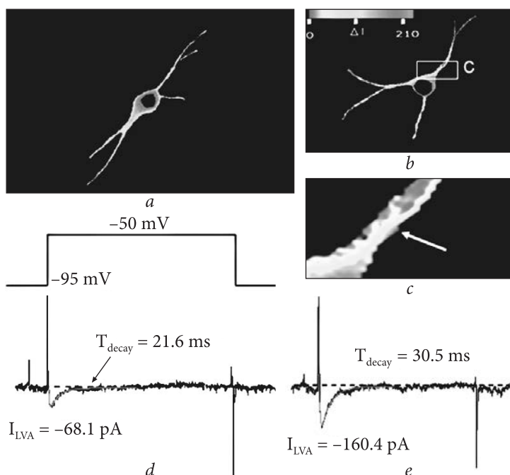
Fig. 3. Control of \text{Ca}^{2+} entry through LVA _f \text{Ca}^{2+} channels in whole-cell configuration: a — \Delta F signal induced by step depolarization in bipolar neuron; b — \Delta F signal induced by step depolarization in multipolar neuron; c — spatial distribution of the "cold" (blue) and "hot" area induced by \text{Ca}^{2+} entry in multipolar neuron; d and e — original LVA _f \text{Ca}^{2+} currents
